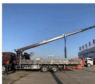
6*4 HOWO STRAIGHT+Auger
